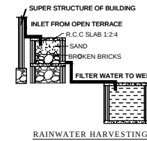
RAINWATER HARVESTING
