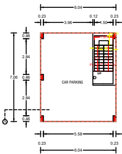
STILT FLOOR PLAN
