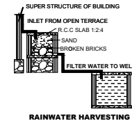
RAINWATER HARVESTING
