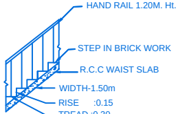
STAIR DETAIL
