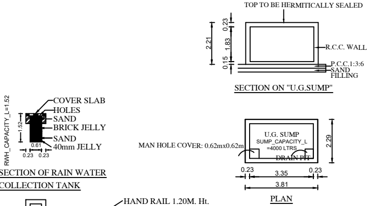
SECTION ON "U.G.SUMP"
