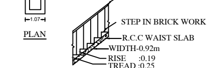
STAIR DETAIL
