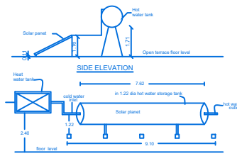
SOLAR WATER HEATER PLANT
