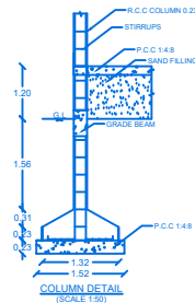
COLUMN DETAIL
