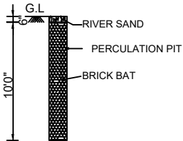
PERCOLATION PIT
