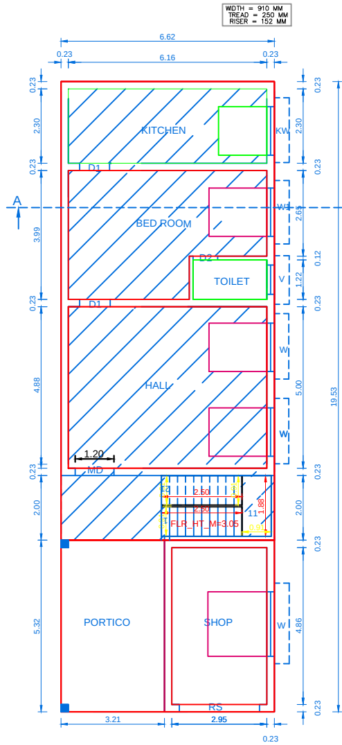
EXG & PROP.GROUND FLOOR PLAN
