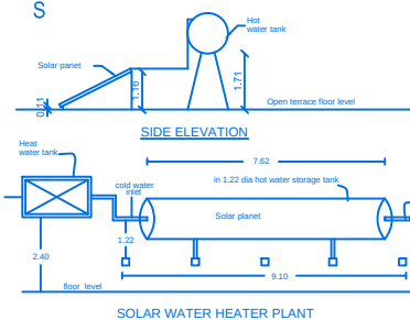
SOLAR WATER HEATER PLANT
