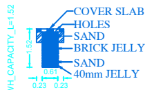
SECTION OF RAIN WATER COLLECTION TANK
