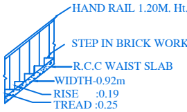
STAIR DETAIL
