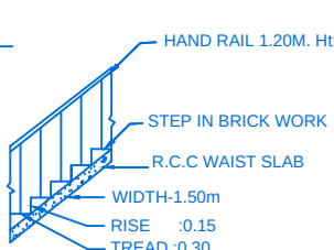
STAIR DETAIL
