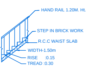
STAIR DETAIL
