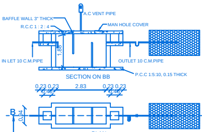
SEPTIC TANK AND TRENCH & U TRAP ADOPTED
