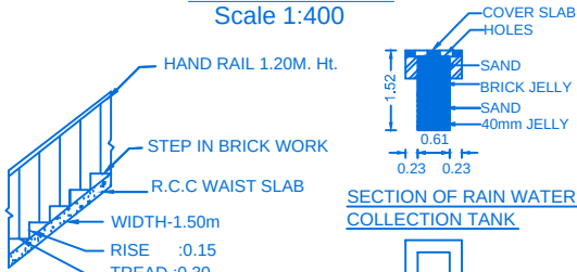
STAIR DETAIL
