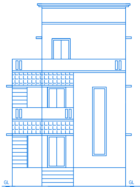
FRONT ELEVATION
