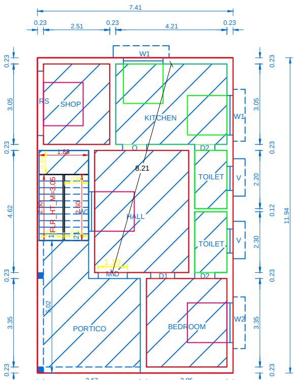
EXG.GROUND FLOOR PLAN
