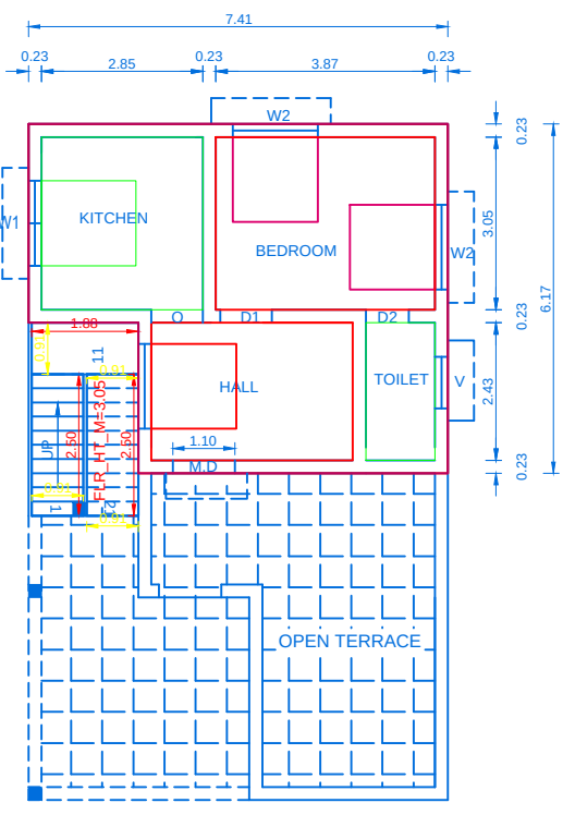
PROP.SECOND FLOOR PLAN
