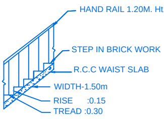
STAIR DETAIL
