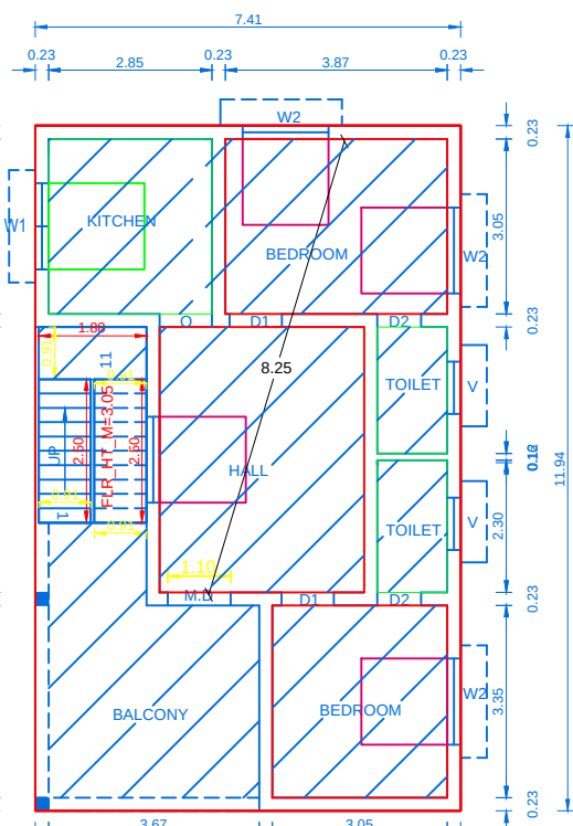
EXG.FIRST FLOOR PLAN
