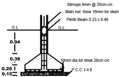
Details of column footing
