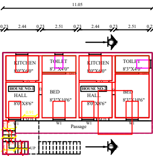
PRO.F.FLOOR PLAN
