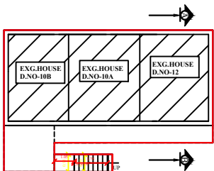
EXG.G.FLOOR PLAN
