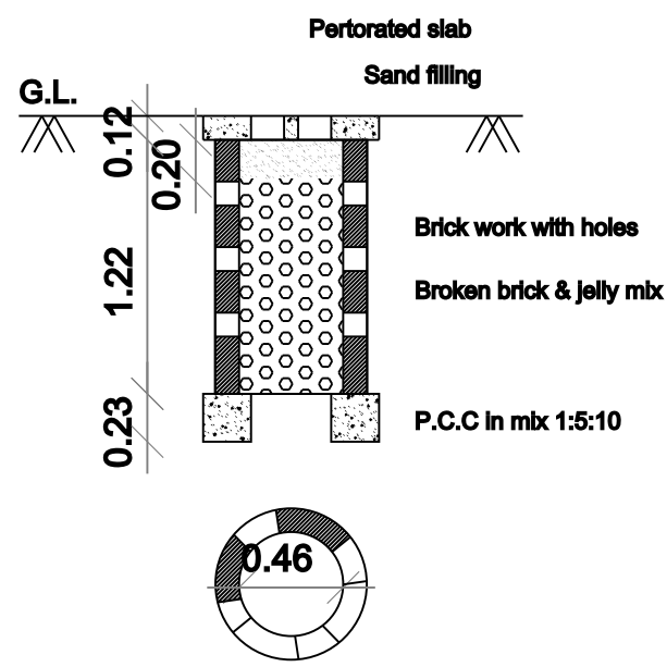
PERCOLATION PIT FOR 30 Sq. m. (Scale:- 1:50)
