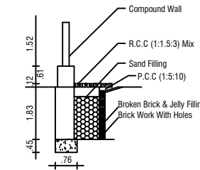
RAIN WATER HARVEST DETAILS
