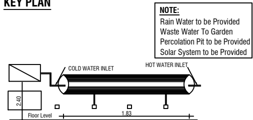
DETAILS OF SOLAR HOT WATER SYSTEM
