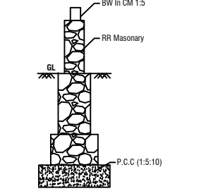
DETAILS OF RR MASONARY
