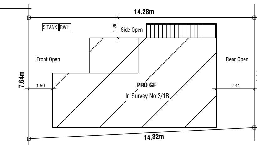
SITE PLAN (1:100)
