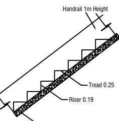
STAIR DETAILS
