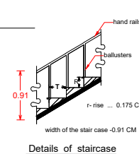
Details of staircase
