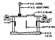
SEC. OF SEPTIC TANK
