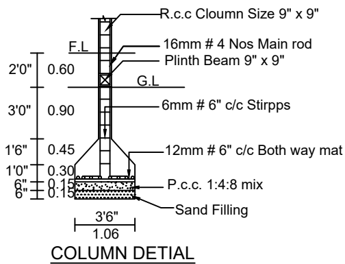
COLUMN DETIAL
