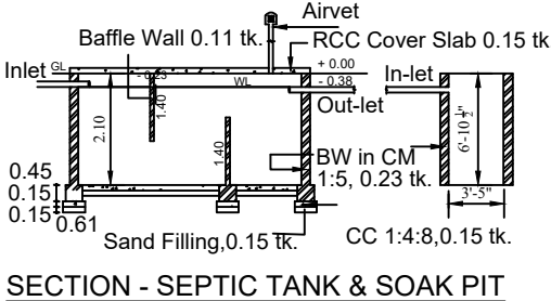
SECTION - SEPTIC TANK & SOAK PIT
