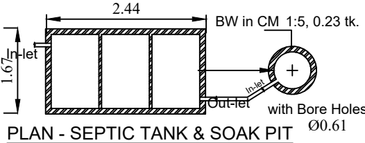
PLAN - SEPTIC TANK & SOAK PIT
