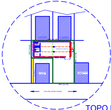
PROPOSED G.F. PLAN
