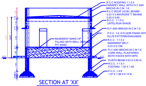
SECTION AT 'XX'
