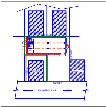
SITE PLAN (Scale 1 :400)
