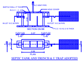
SEPTIC TANK AND TRENCH & U TRAP ADOPTED
