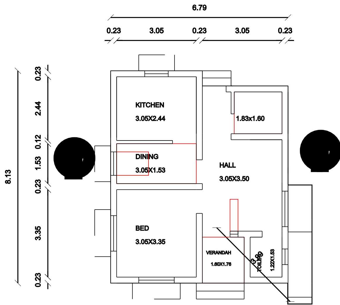
GORUND FLOOR PLAN
