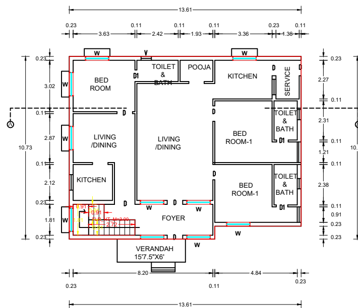
EXG. GROUND FLOOR PLAN
