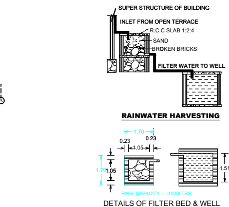
DETAILS OF FILTER BED & WELL
