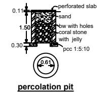
PERCOLATION PIT
