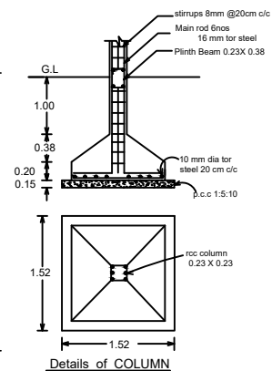
DETAILS OF COLUMN
