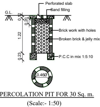
RAINWATER HARVESTING
