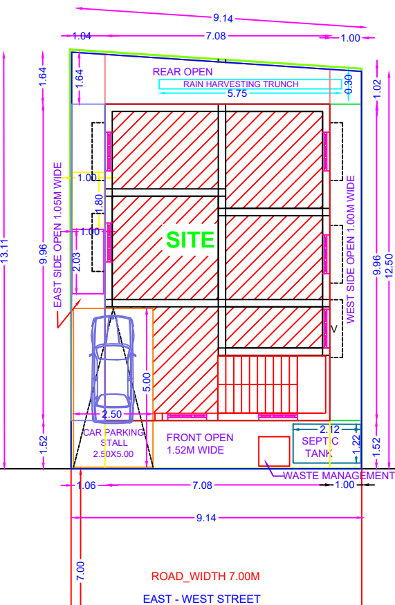
SITE PLAN
