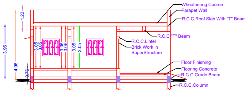
SECTION ON "PQ"
