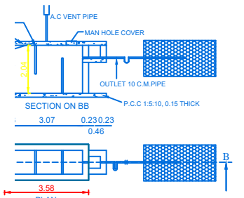
SEPTIC TANK AND TRENCH & U TRAP ADOPTED
