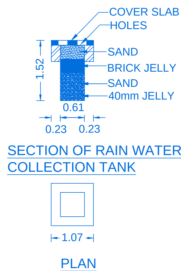
PLAN
