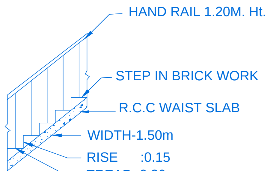
STAIR DETAIL
