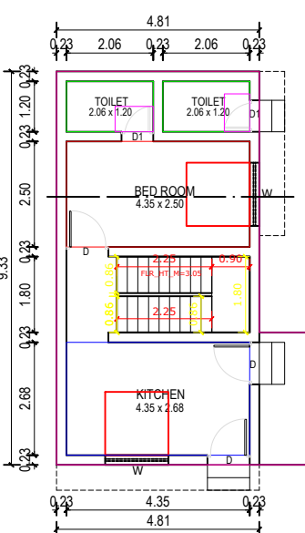
GF PLAN
