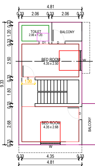
FF PLAN
