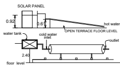
Details of solar water heating system
