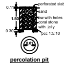
percolation pit
