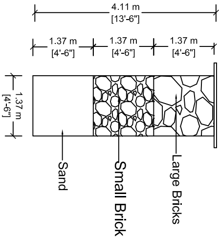
SECTION OF RAIN WATER COLLECTION PITS (NTS)
