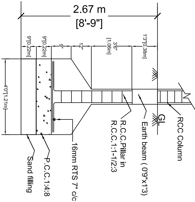
FOUNDATION DETAILS
