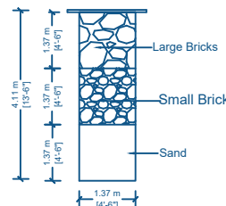
SECTION OF RAIN WATER COLLECTION PITS (NTS)
