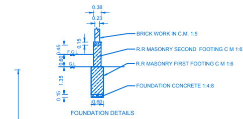
FOUNDATION DETAILS
