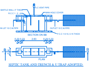
SEPTIC TANK AND TRENCH & U TRAP ADOPTED.
