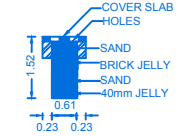
SECTION OF RAIN WATER COLLECTION TANK
