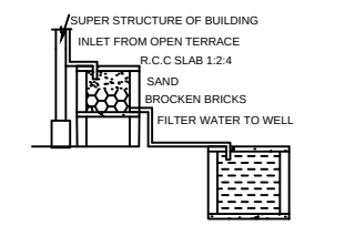
RAINWATER HARVESTING
