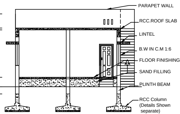
CROSS SECTION VIEW AB
