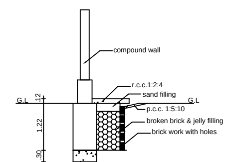
PLINTH BOUNDARY PERCOLATION PIT
