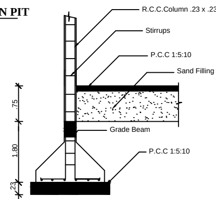
COLUMN DETAIL
