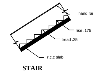
STAIR
