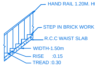
STAIR DETAIL
