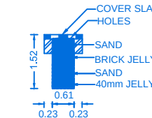
SECTION OF RAIN WATER COLLECTION TANK
