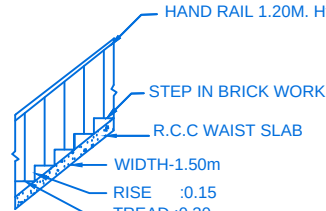
STAIR DETAIL
