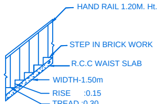
STAIR DETAIL
