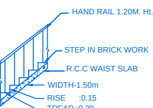
STAIR DETAIL
