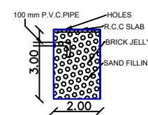
SECTION OF RAIN WATER COLLECTING TANK
