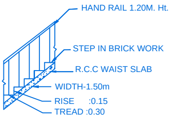
STAIR DETAIL
