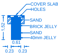
SECTION OF RAIN WATER COLLECTION TANK
