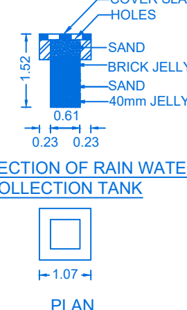
SECTION OF RAIN WATER COLLECTION TANK
