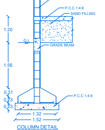
COLUMN DETAIL (SCALE 1:50)
