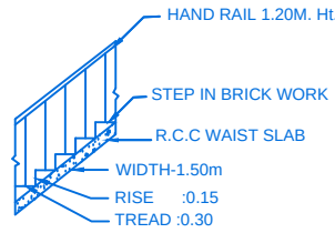
STAIR DETAIL
