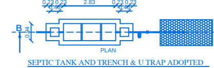
SEPTIC TANK AND TRENCH & U TRAP ADOPTED
