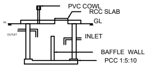
SEC. OF SEPTIC TANK
