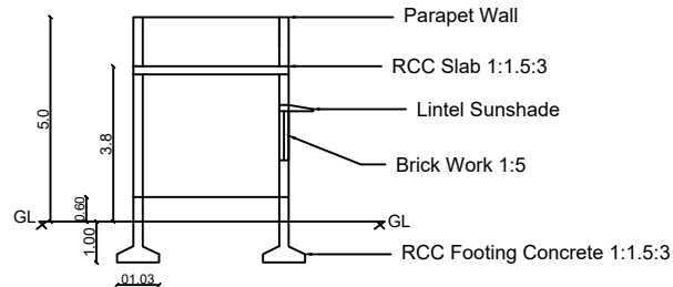
SECTION A- A VIEW
