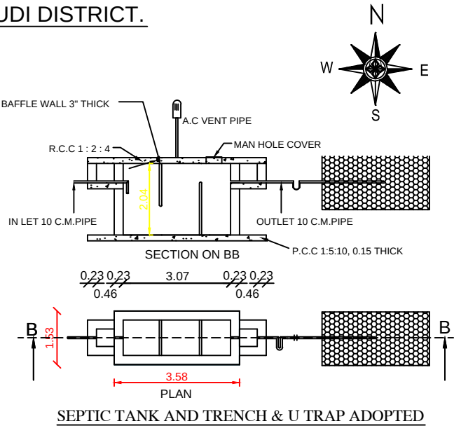
SEPTIC TANK AND TRENCH & U TRAP ADOPTED
