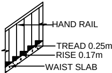
STAIR CASE DETAIL
