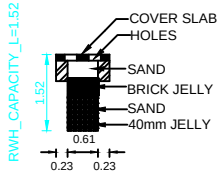
SECTION OF RAIN WATER COLLECTION TANK
