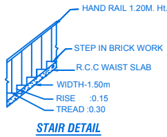
STAIR DETAIL
