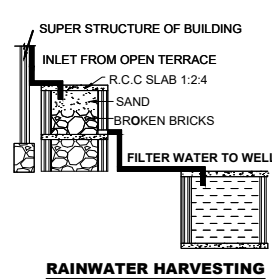
RAINWATER HARVESTING
