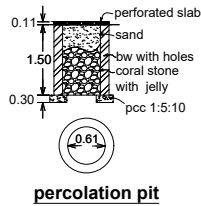
percolation pit
