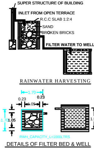
DETAILS OF FILTER BED & WELL
