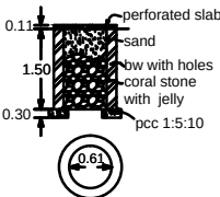
percolation pit
