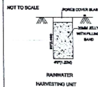
RAINWATER HARVESTING UNIT
