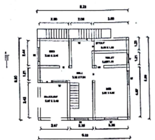
PRO.FIRST FLOOR PLAN
