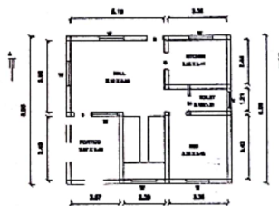
PRO.GROUND FLOOR PLAN
