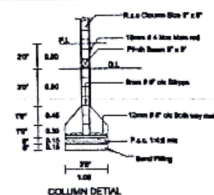
COLUMN DETAIL
