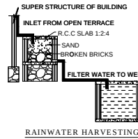
RAINWATER HARVESTING
