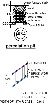
DETAILS OF STAIRCASE
