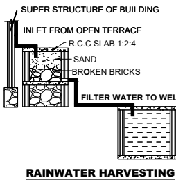
RAINWATER HARVESTING
