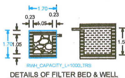
DETAILS OF FILTER BED & WELL
